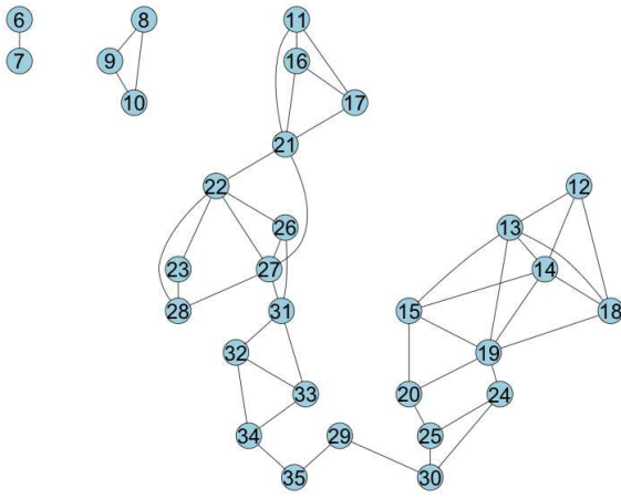
Fig. 6: Connected components for parcel p_2 with h = 5
