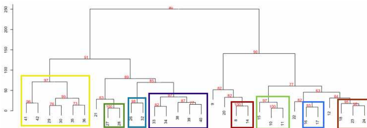
Fig. 11: Dendrogram representing parcel p_1 clustering
